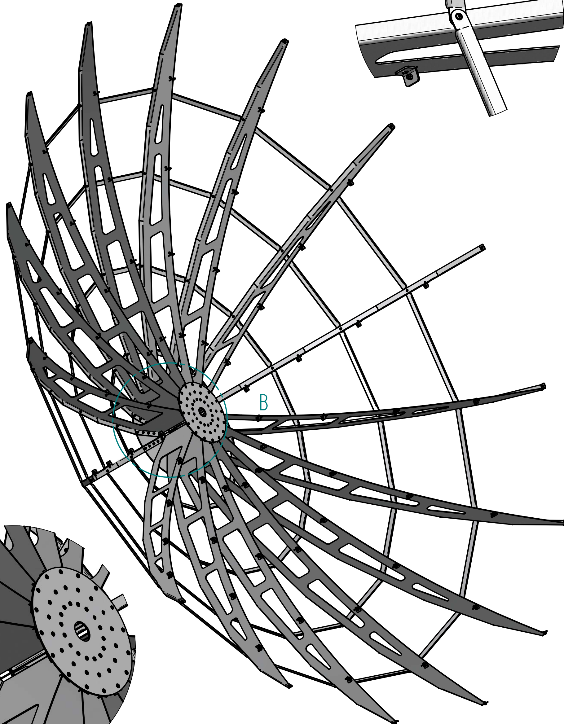
DETAIL C
