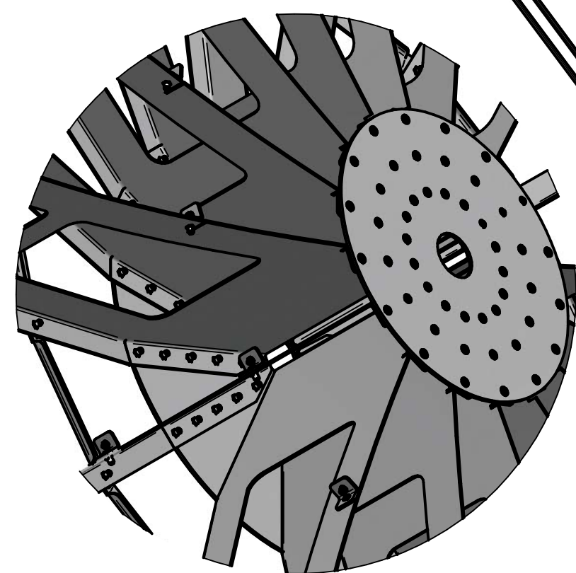
DETAIL B
